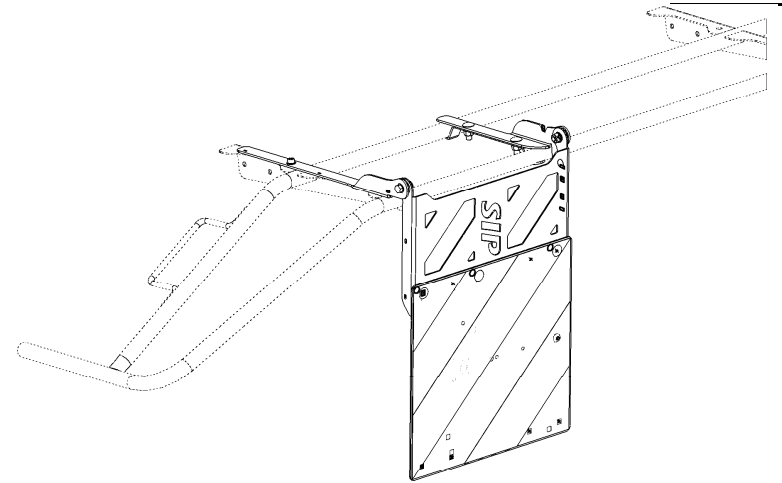
DETAIL D SCALE 1 : 10
