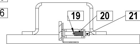
SECTION C-C SCALE 1 : 5 OPTICUT DISC 300 S ALP=+041
