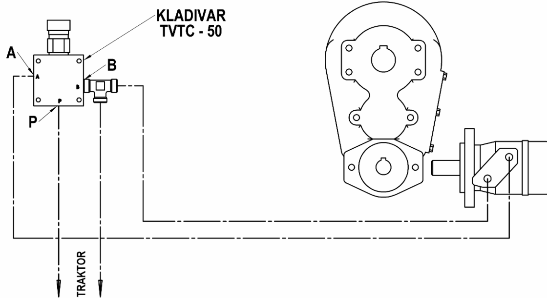
Hydraulik motor bindung scheme Binding scheme of hydraulic motor
